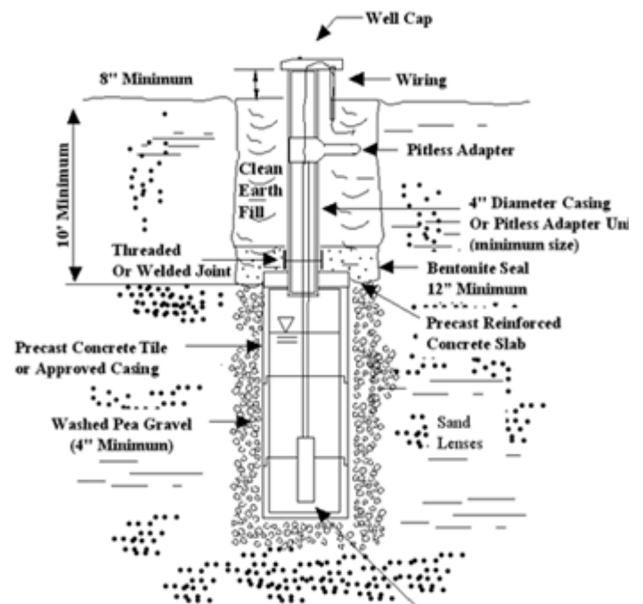
Figure 1 - Bored or Dug Well - Buried Slab Construction
