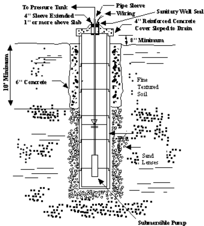
Figure 2 - Bored Well With Concrete Collar
